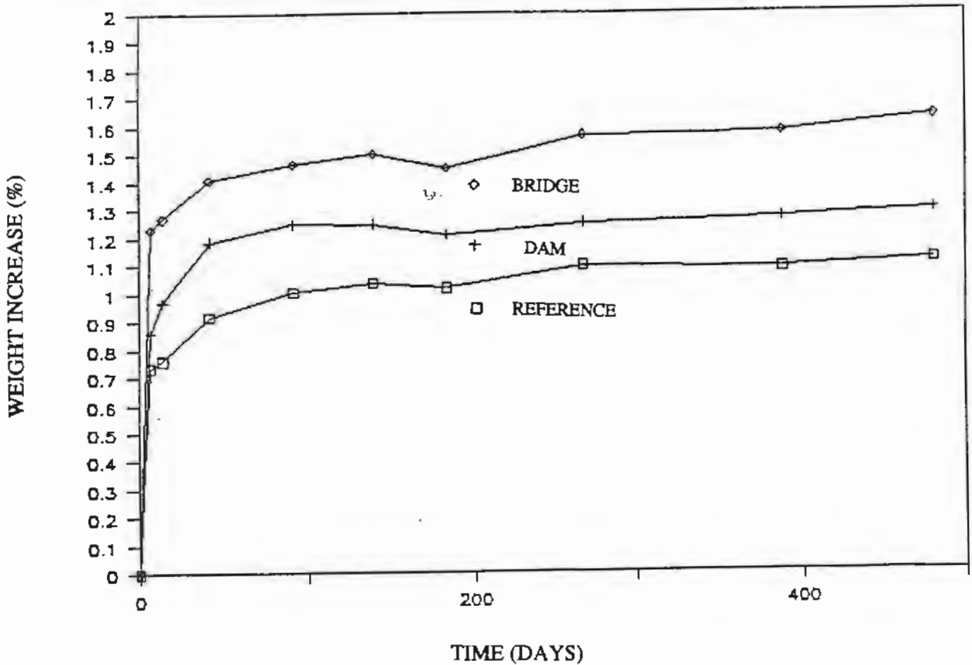
Figure 4: Weight increase for the expansion specimens
