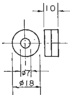
Fig. 8 Special expanding steel disc for the CAPO-TEST system. (Dimensions in mm).
