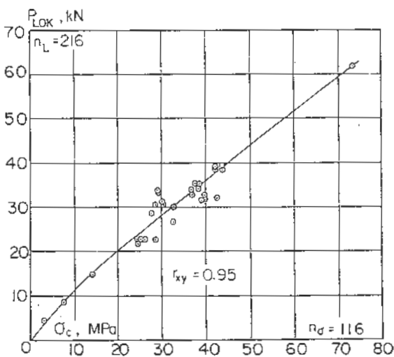
Fig. 10 and 11 Calibration curves from LOK-TEST and CAPO-TEST investigations carried out in 1979 (Technical University of Denmark, Department of Structural Engineering).
