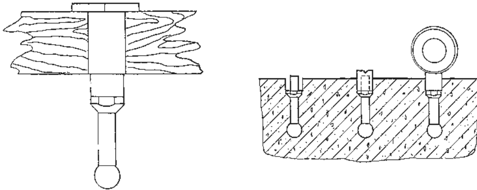
Fig. 1 Specially shaped steel rods with spherically thickened ends for the Russian pullout testing system (Volf and Gershberg, 1934/38).
