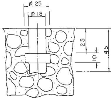
Fig. 7 Hole and groove drilled out for the so-called CAPO-TEST pullout system. (Dimensions in mm).
