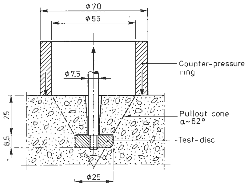
Fig. 6 Test set-up for the so-called LOK-TEST pullout system. (Dimensions in mm).
