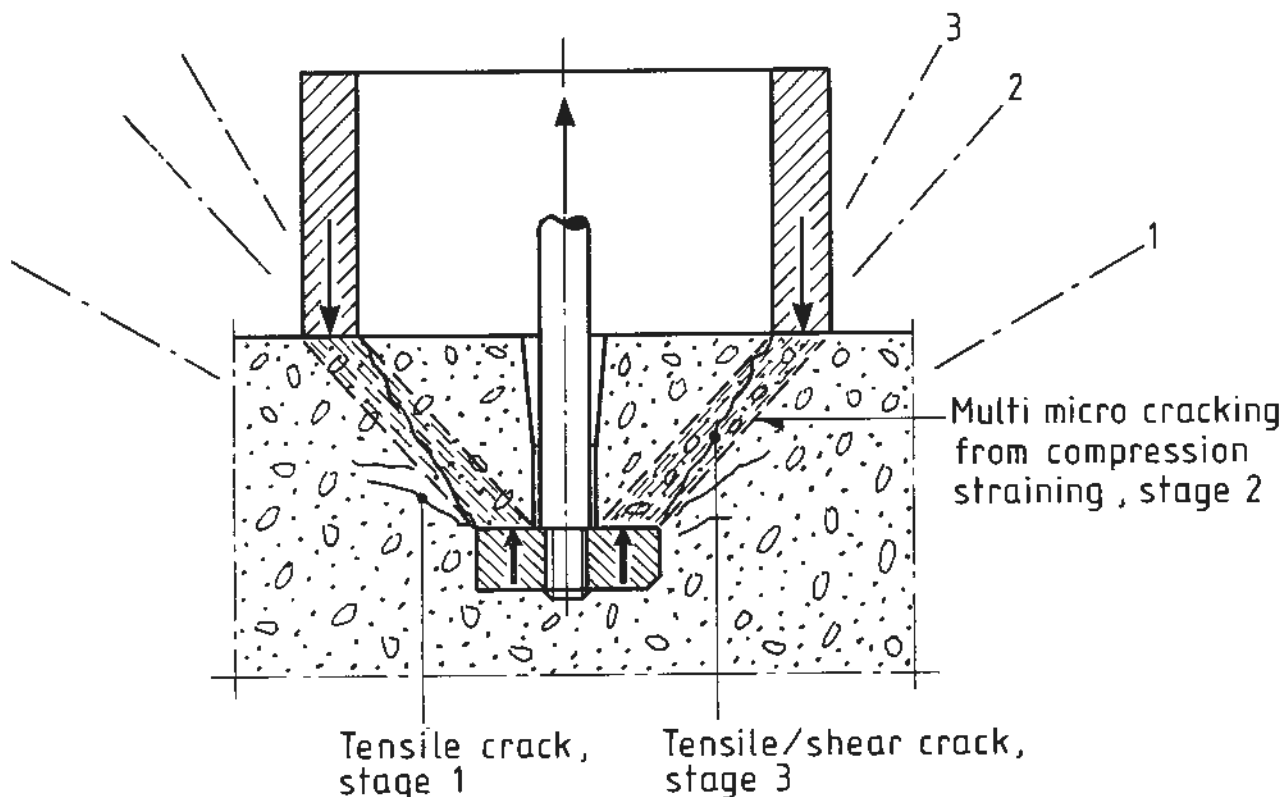
Fig. 13 The three different stages of internal cracking in the concrete during pull-out loading.
