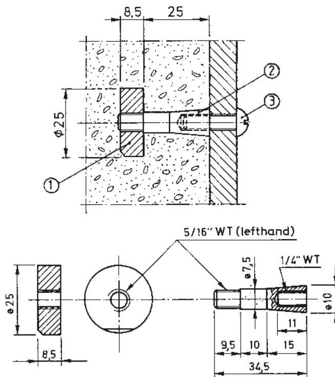
Fig. 5 Pullout disc and bolt fixed on inside of form before casting the concrete.
