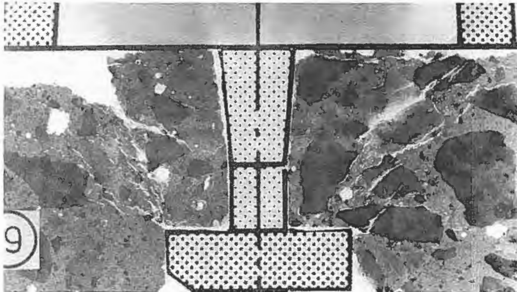
Fig. 12 Crack analysis of pullout test de-loaded from peak of load/displacement curve. Tensile cracking stage No. 1 is seen to the left and multi micro cracking stage 2 to the right. Pullout crack stage 3 has not yet been formed.
