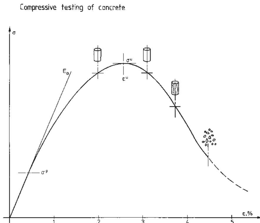
Fig. 14 Stress-strain curve from uniaxial compressive test on plain concrete.
