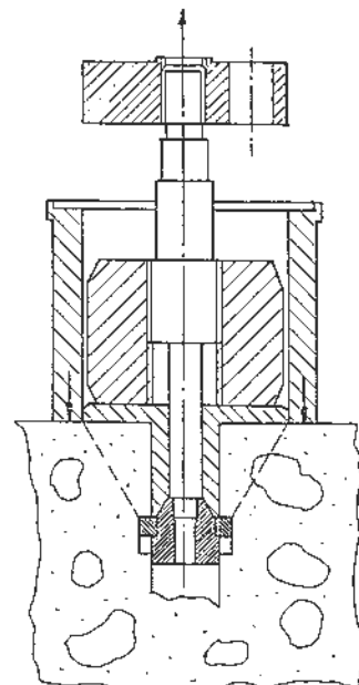
Fig. 9 Test set-up for the CAPO-TEST system.
